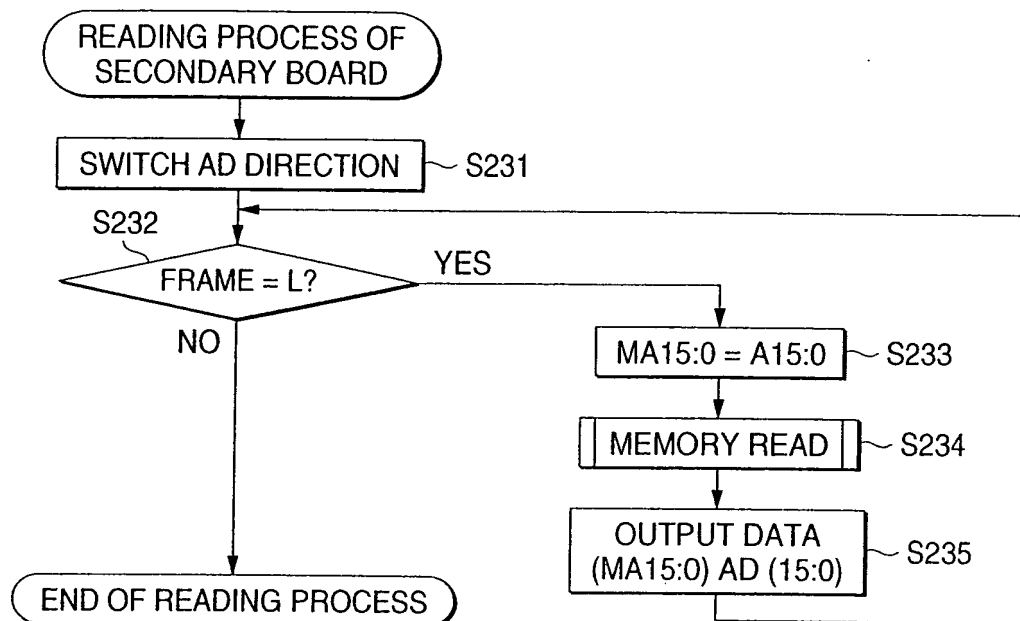
FIG. 21 PRIOR ART
